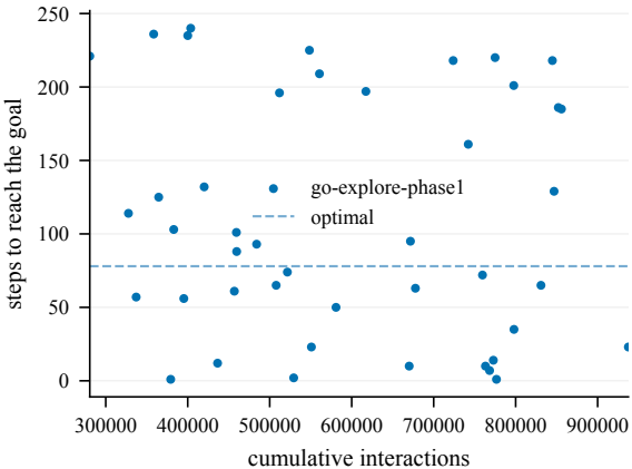
Steps to goal (train) -- Nested1-50@4000
