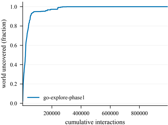
Cumulative coverage -- Nested1-50@4002
