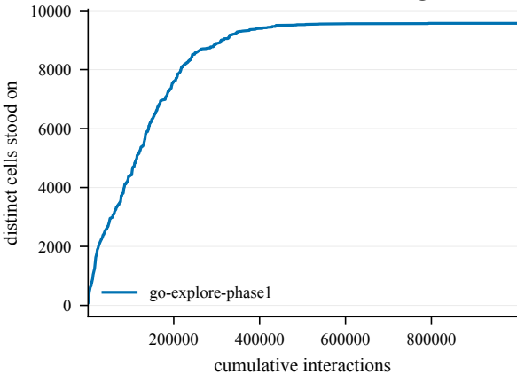
States discovered -- Nested2-100@4001
