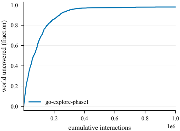
Cumulative coverage -- Nested2-100@4002
