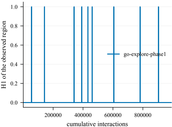
Discovered topology -- Nested2-50@4000
