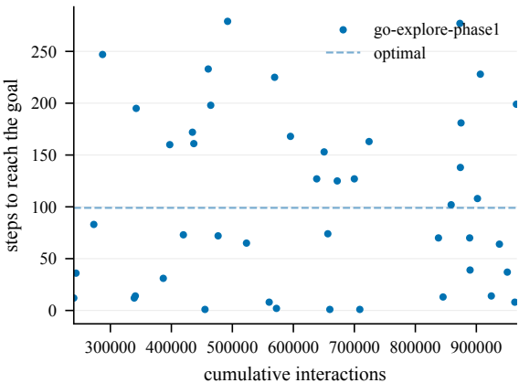
Steps to goal (train) -- Nested2-50@4000
