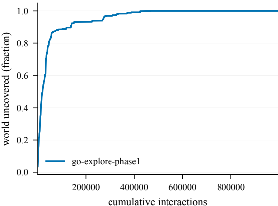
Cumulative coverage -- Nested2-50@4001
