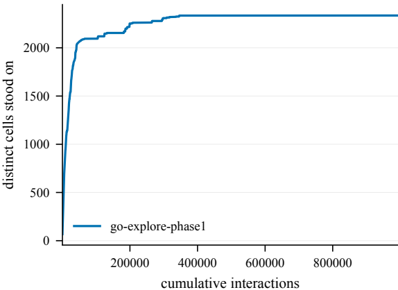
States discovered -- Nested2-50@4002
