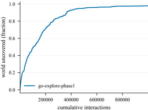
Cumulative coverage -- Nested3-100@4000
