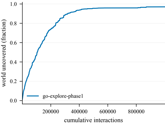
Cumulative coverage -- Nested3-100@4001
