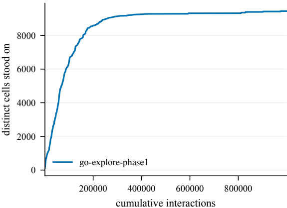
States discovered -- Nested3-100@4002
