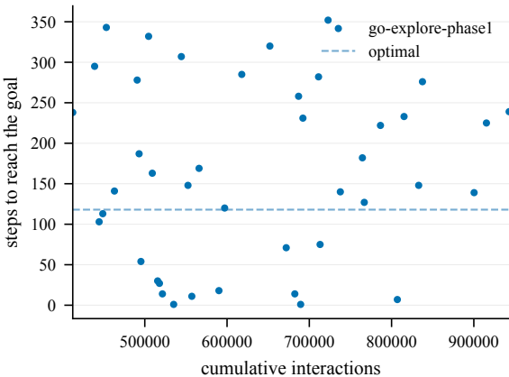
Steps to goal (train) -- Nested3-50@4000
