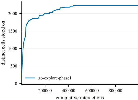
States discovered -- Nested3-50@4000
