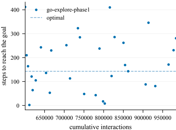
Steps to goal (train) -- Nested3-50@4001
