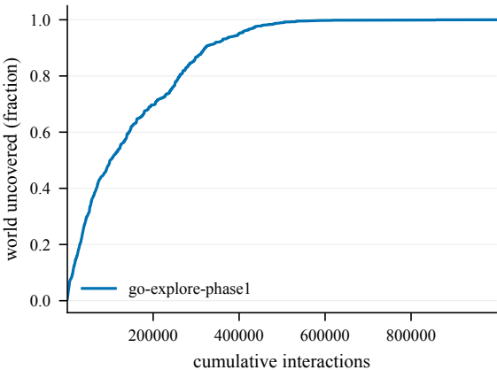
Cumulative coverage -- ShapeCi-100@4000
