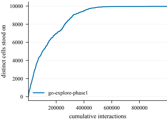
States discovered -- ShapeCi-100@4000
