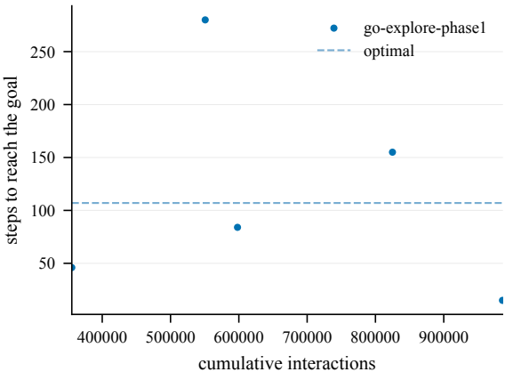
Steps to goal (train) -- ShapeCi-100@4001
