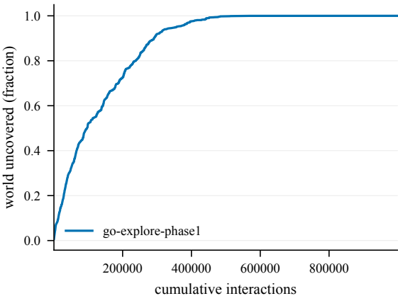
Cumulative coverage -- ShapeCi-100@4002
