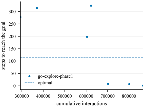
Steps to goal (train) -- ShapeCi-100@4002
