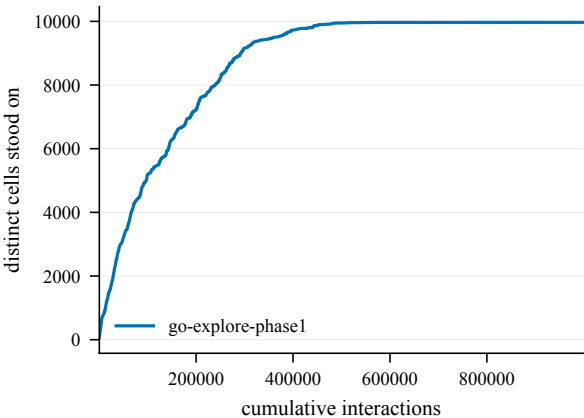
States discovered -- ShapeCi-100@4002
