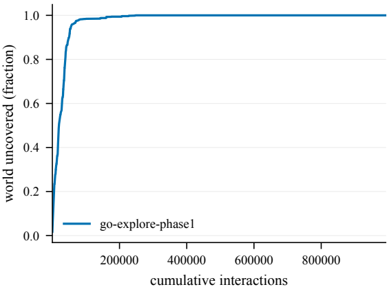
Cumulative coverage -- ShapeCi-50@4000
