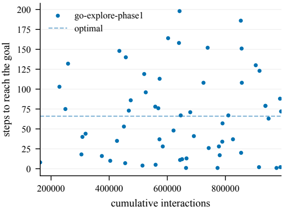
Steps to goal (train) -- ShapeCi-50@4000
