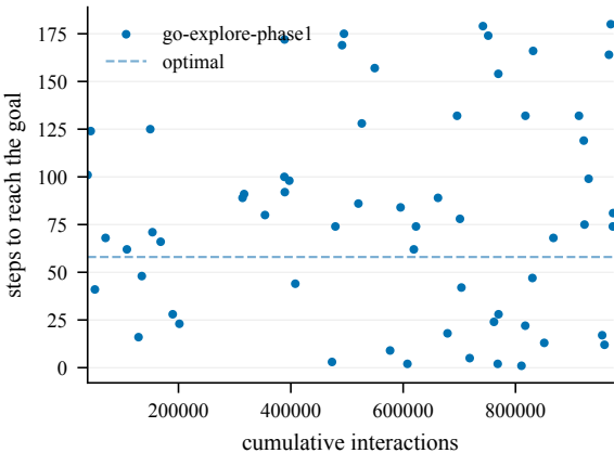
Steps to goal (train) -- ShapeCi-50@4001
