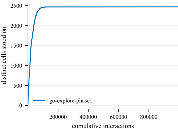
States discovered -- ShapeCi-50@4001
