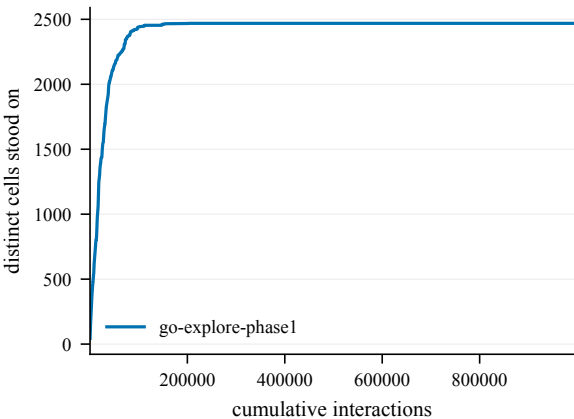
States discovered -- ShapeCi-50@4002
