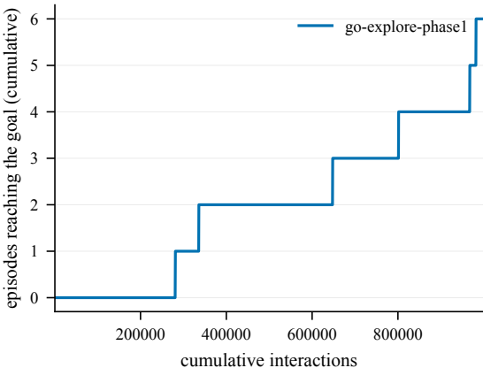
Goal reached -- ShapeSq-100@4000
