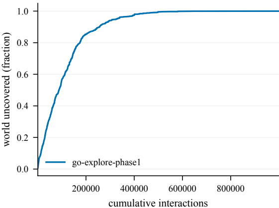
Cumulative coverage -- ShapeSq-100@4000
