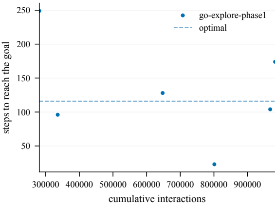
Steps to goal (train) -- ShapeSq-100@4000
