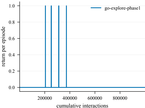
Return -- ShapeSq-100@4001
