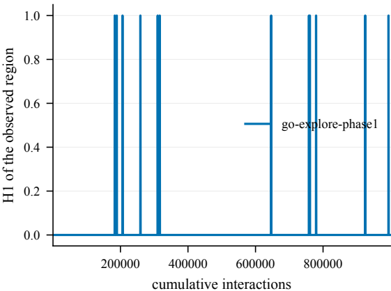
Discovered topology -- ShapeSq-100@4001
