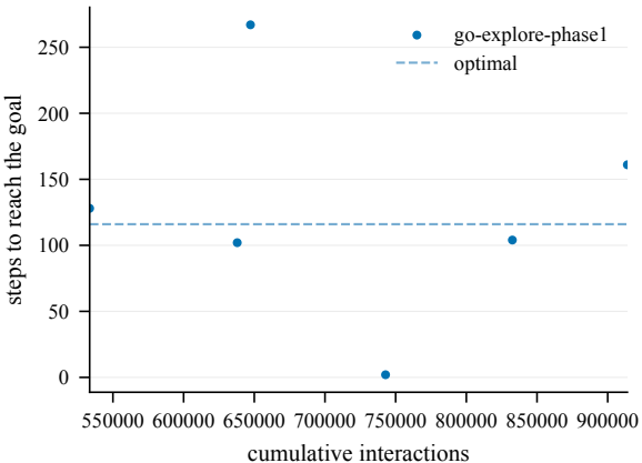
Steps to goal (train) -- ShapeSq-100@4002
