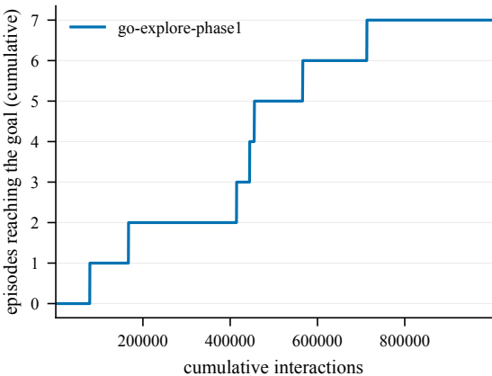
Goal reached -- ShapeSt-100@4000
