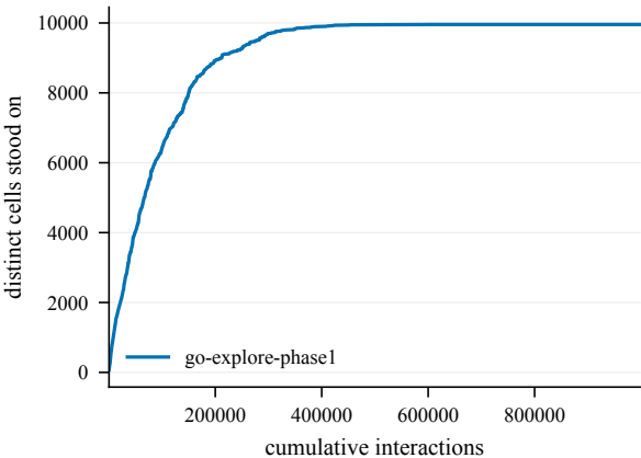
States discovered -- ShapeSt-100@4000
