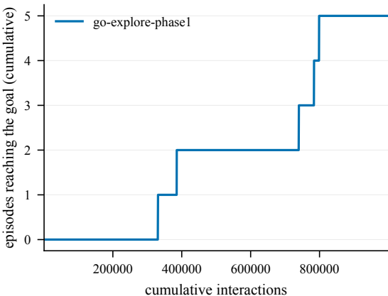
Goal reached -- ShapeSt-100@4001
