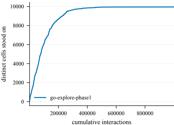
States discovered -- ShapeSt-100@4001
