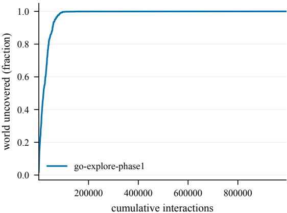
Cumulative coverage -- ShapeSt-50@4000
