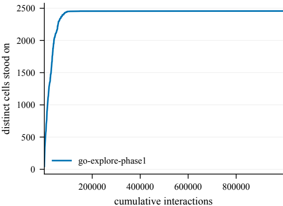
States discovered -- ShapeSt-50@4000
