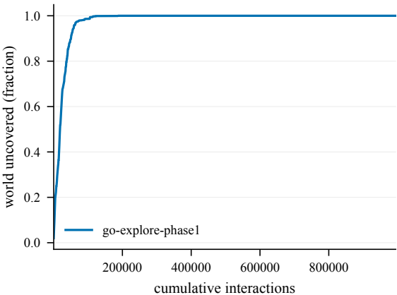
Cumulative coverage -- ShapeSt-50@4002
