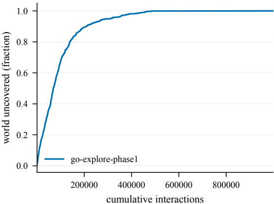
Cumulative coverage -- ShapeTr-100@4000
