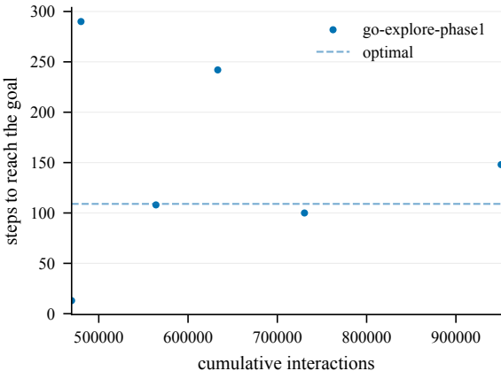
Steps to goal (train) -- ShapeTr-100@4000
