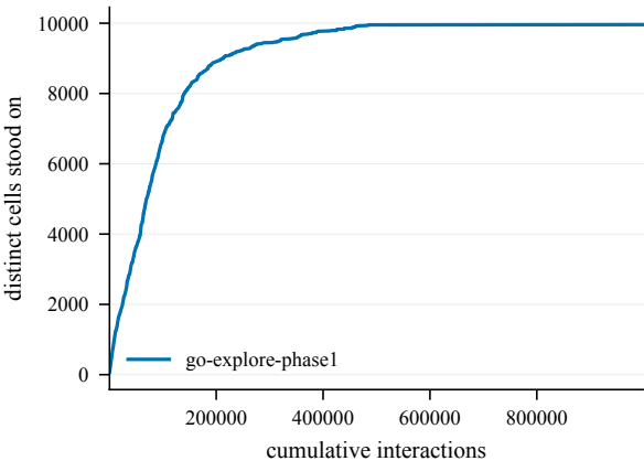
States discovered -- ShapeTr-100@4000
