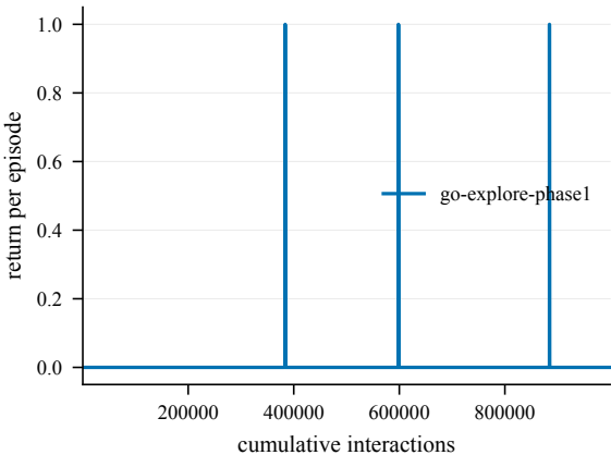
Return -- ShapeTr-100@4001
