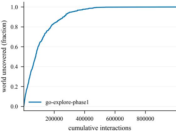
Cumulative coverage -- ShapeTr-100@4001
