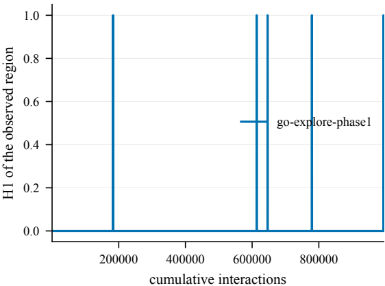
Discovered topology -- ShapeTr-50@4000
