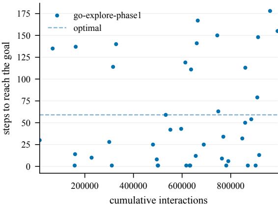
Steps to goal (train) -- ShapeTr-50@4000
