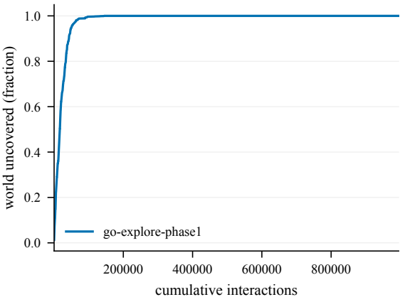
Cumulative coverage -- ShapeTr-50@4001
