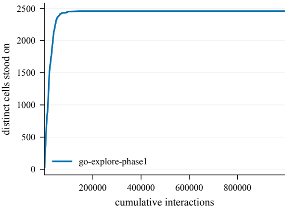
States discovered -- ShapeTr-50@4001
