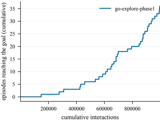
Goal reached -- ShapeTr-50@4002
