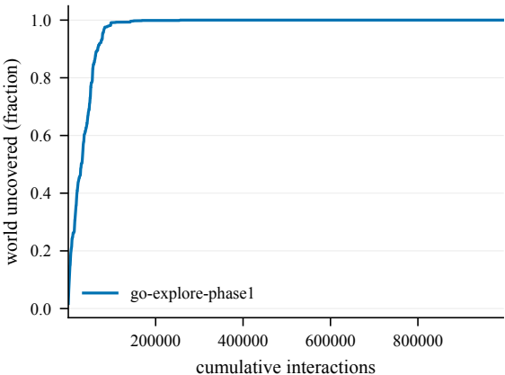
Cumulative coverage -- ShapeTr-50@4002
