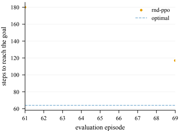
Steps to goal (eval) -- ShapeTr-50@4002
